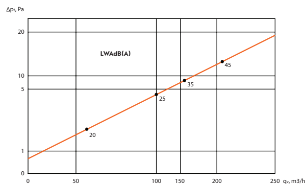
LINEO PRO 125 PUZZLE, 20 mm slot (extract air)
