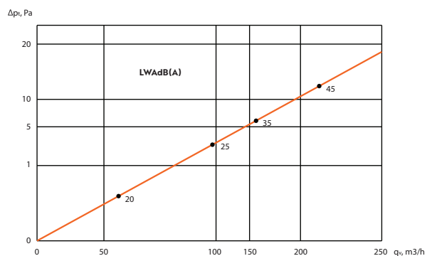
LINEO PRO 125 PUZZLE, 20 mm slot (supply air)
